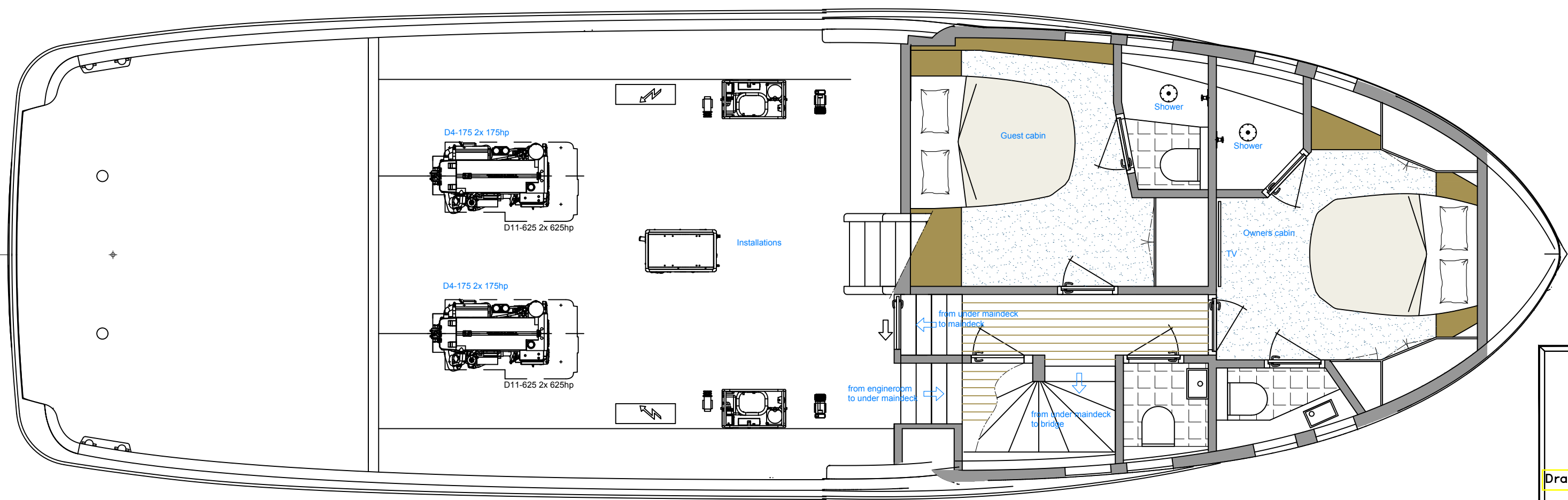
UNDER MAINDECK
